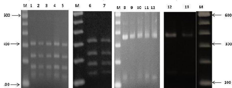
Figure 2 - Electrophoresis of PCR products of ITS1-ITS4 (2% agarose gel). Fragments were obtained after enzymatic digestion with Hae III (Lines 1-7) and Hinf I (Lines 8-13). Line M: Molecular weight 100 bp (Invitrogen TM), Lines 1 and 8: L32, Lines 2 and 9: L34, Lines 3 and 10: L36, Lines 4 and 11: L38, Lines 5 and 12: B32, Lines 6 and 7: PE-2, Lines 7 and 13: S. cerevisiae (CEFAR CCCD-SS001)
